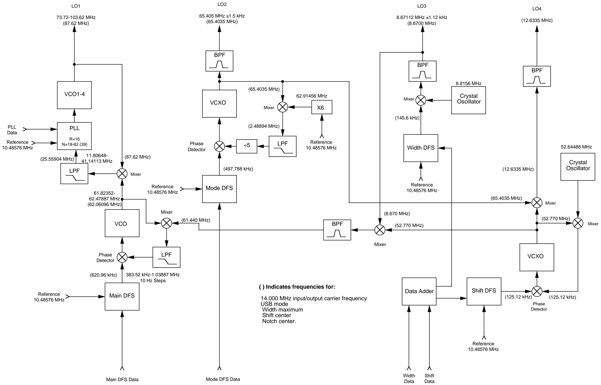
FT-1000D Local Unit Block Diagram
